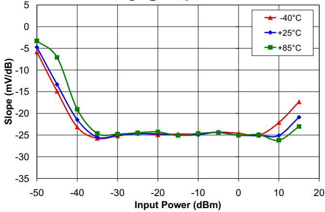
Slope Vs Input Power Over Temperature Range @ Freq 5000MHz
