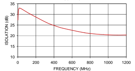
ZX10-2-12+ ISOLATION
