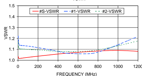
ZX10-2-12+ VSWR
