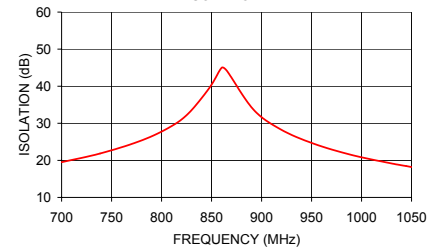
ZN2PD-920W+ ISOLATION
