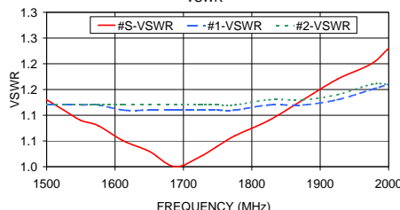
ZN2PD-1900W VSWR
