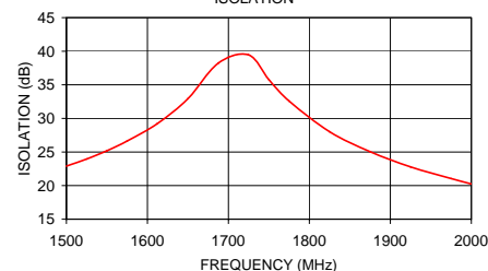
ZN2PD-1900W ISOLATION
