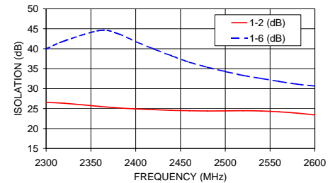
ZC10PD-26 ISOLATION
