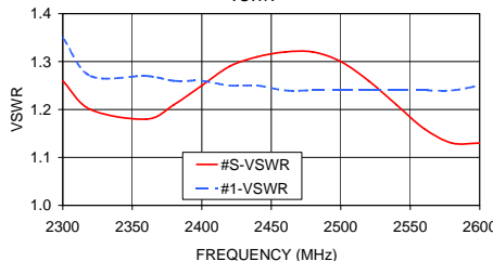
ZC10PD-26 VSWR
