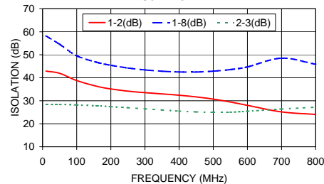
ZBSC-8-82+ ISOLATION
