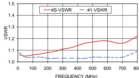
ZBSC-8-82+ VSWR
