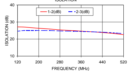
ZBSC-5-1 ISOLATION
