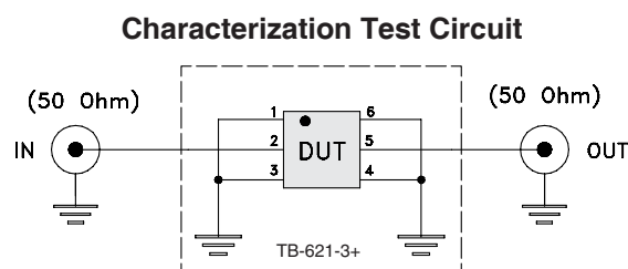
Fig 1. Block diagram of Test Circuit used for characterization, Test board TB-621-3+ Conditions: Attenuation, VSWR: Pin=-10 dBm
