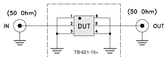
Fig 1. Block diagram of Test Circuit used for characterization, Test board TB-621-15+ Conditions: Attenuation, VSWR: Pin=-10 dBm
