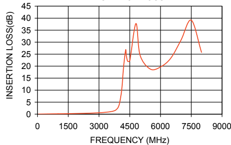
VLF-3400+ INSERTION LOSS
