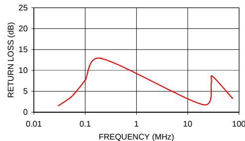
T16-6T-KK81 INPUT RETURN LOSS
