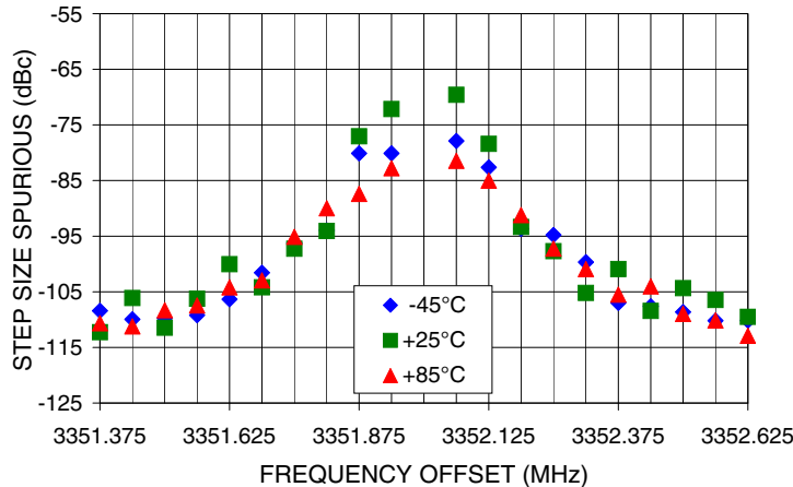
0.5 STEP SIZE & STEP SIZE SPURIOUS Vs FREQ. OFFSET @ F car = 3352MHz
