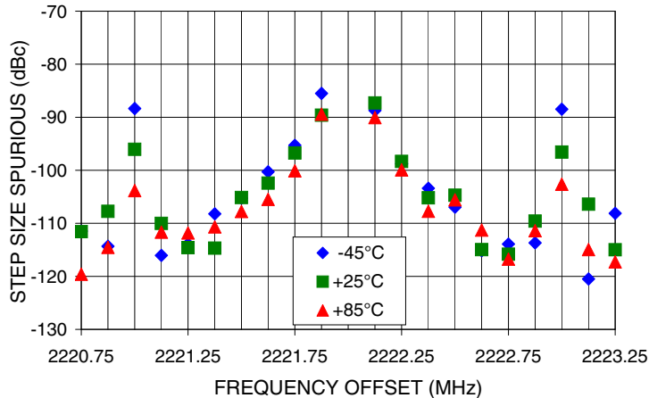
0.5 STEP SIZE & STEP SIZE SPURIOUS Vs FREQ. OFFSET @ Fcar = 2222MHz
