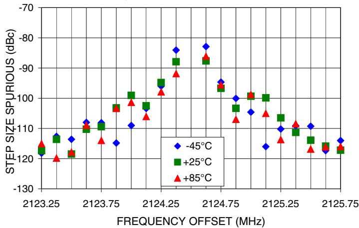
0.5 STEP SIZE & STEP SIZE SPURIOUS Vs FREQ. OFFSET @ Fcar = 2124.5MHz
