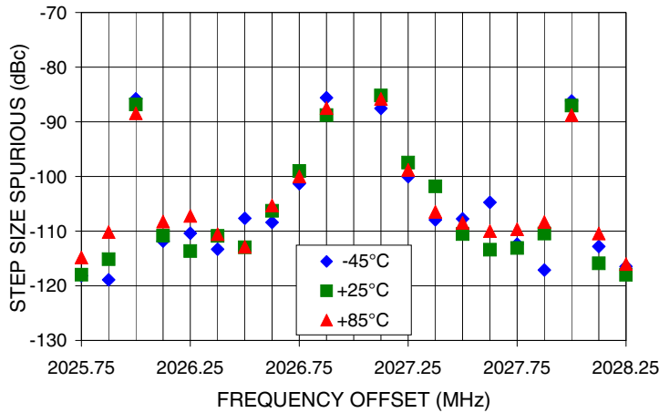
0.5 STEP SIZE & STEP SIZE SPURIOUS Vs FREQ. OFFSET @ Fcar = 2027MHz
