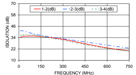
SCP-4-1W-75 ISOLATION
