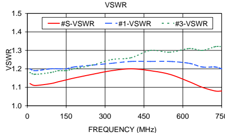
SCP-4-1W-75 VSWR
