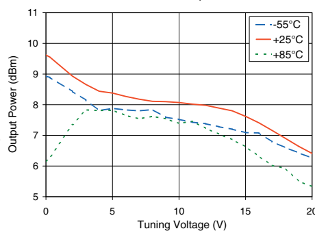
ROS-1300+ Power Output
