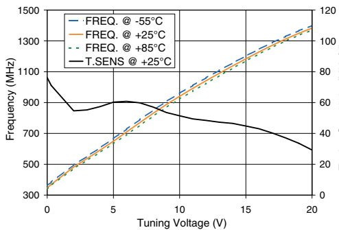
ROS-1300+ Frequency and Tuning Sensitivity
