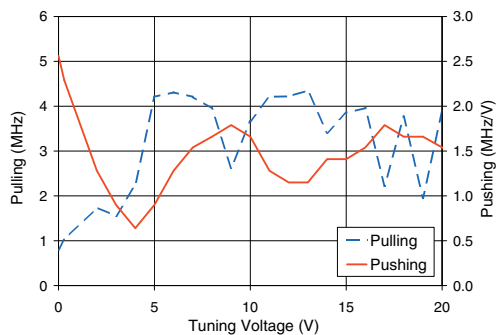
ROS-1300+ Frequency Pulling & Pushing (Vcc ± 5%)
