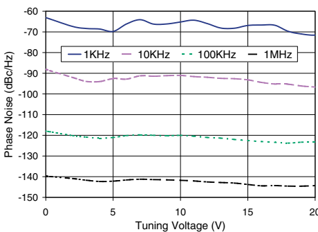
ROS-1300+ Phase Noise Vs. Tuning Voltage
