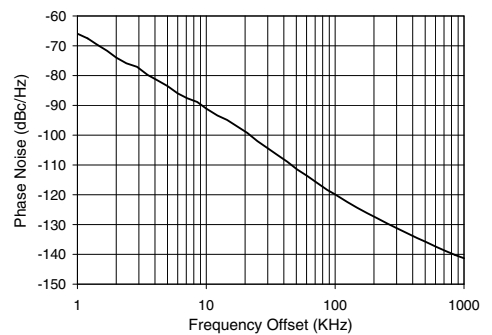
ROS-1300+ Phase Noise
