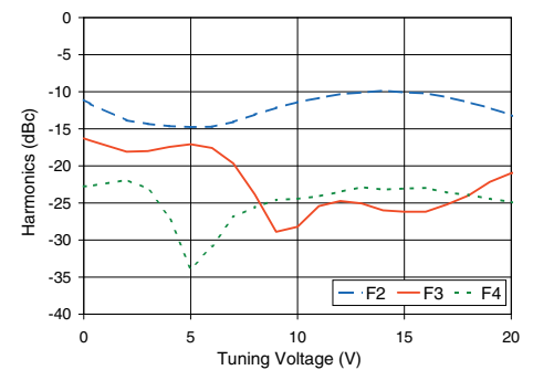
ROS-1300+ Harmonics Level
