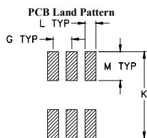
Suggested Layout, Tolerance to be within ±.002
