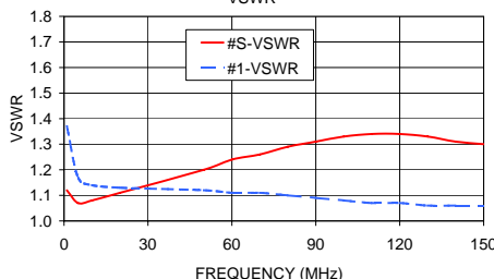
PSC-10-1 VSWR
