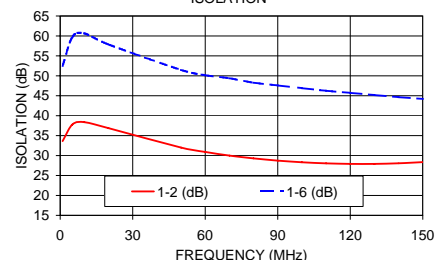
PSC-10-1 ISOLATION
