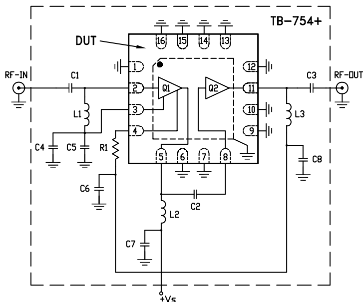
Fig 1. Application and Characterization circuit Note: This block diagram is used for characterization. (DUT soldered on Mini-Circuits Characterization test board TB-754+) Gain, Return loss, Output power at 1dB compression (P1 dB), output IP3 (OIP3) and noise figure measured using Agilent's N5242A PNA-X microwave network analyzer.
