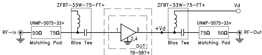
Fig 1. Block Diagram of Test Circuit used for characterization. (DUT tested on Mini-Circuits Characterization test board TB-587+) Gain, Return loss, Output power at 1dB compression (P1 dB) , output IP3 (OIP3), output IP2 (OIP2) and noise figure measured using Agilent's N5242A PNA-X microwave network analyzer.
