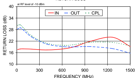
PDC-10-54 RETURN LOSS
