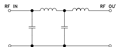
electrical schematic
