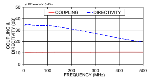
LRDC-10-1J COUPLING & DIRECTIVITY
