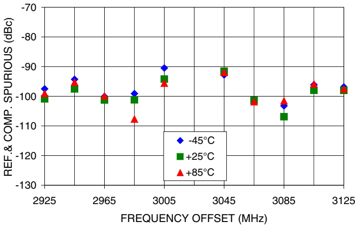
REFERENCE & COMPARISON SPURIOUS Vs FREQ. OFFSET @ Fcar = 3025MHz
