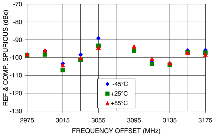
REFERENCE & COMPARISON SPURIOUS Vs FREQ. OFFSET @ Fcar = 3075MHz
