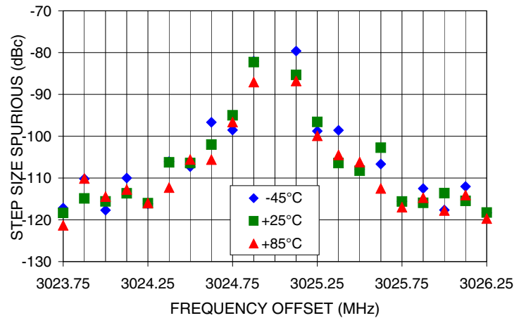
0.5 STEP SIZE & STEP SIZE SPURIOUS Vs FREQ. OFFSET @ Fcar = 3025MHz
