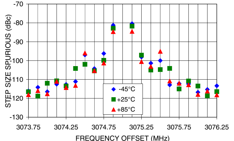
0.5 STEP SIZE & STEP SIZE SPURIOUS Vs FREQ. OFFSET @ Fcar = 3075MHz
