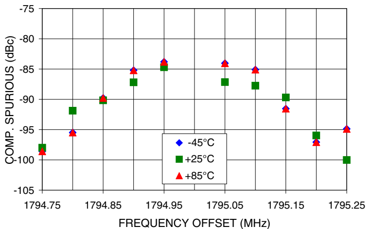
COMPARISON SPURIOUS Vs FREQ. OFFSET @ Fcar = 1795MHz
