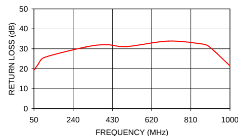
JTX-2-10T INPUT RETURN LOSS
