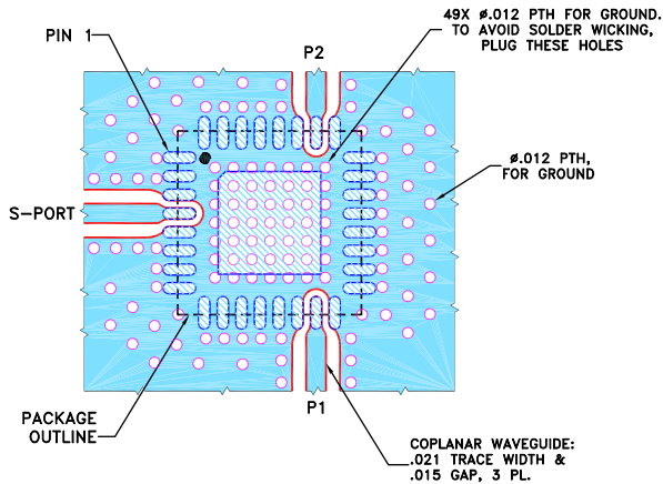
Demo Board MCL P/N: TB-880+ Suggested PCB Layout (PL-488)
