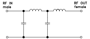
electrical schematic
