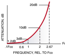
TYPICAL FREQUENCY RESPONSE
