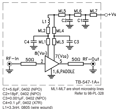
Fig 1. Block Diagram of Test Circuit used for characterization. (DUT soldered on Mini-Circuits Characterization Test Board TB-547-1A+) Gain, Output power at 1dB compression (P1dB), Noise Figure, Output IP3 (OIP3) are measured using Agilent's N5242A PNA-X microwave network analyzer.
