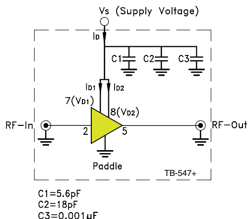
Fig 1. Block Diagram of Test Circuit used for characterization. (DUT soldered on Mini-Circuits Characterization Test Board TB-547+) Gain, Output power at 1dB compression (P1dB), Noise Figure, Output IP3 (OIP3) are measured using Agilent's N5242A PNA-X microwave network analyzer.
