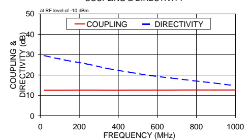
ADC-12-4-75 COUPLING & DIRECTIVITY
