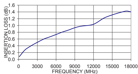
086-14SMR+ INSERTION LOSS
