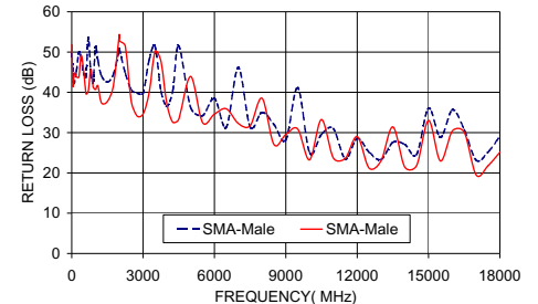
086-14SM+ RETURN LOSS
