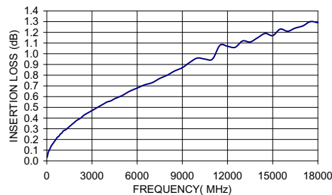
086-14SM+ INSERTION LOSS
