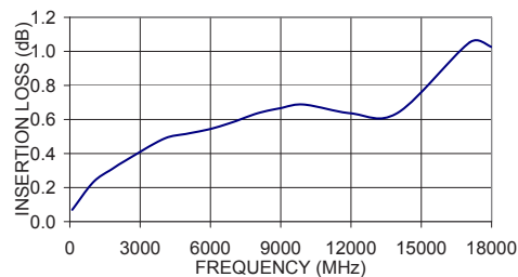
086-10SMR+ INSERTION LOSS
